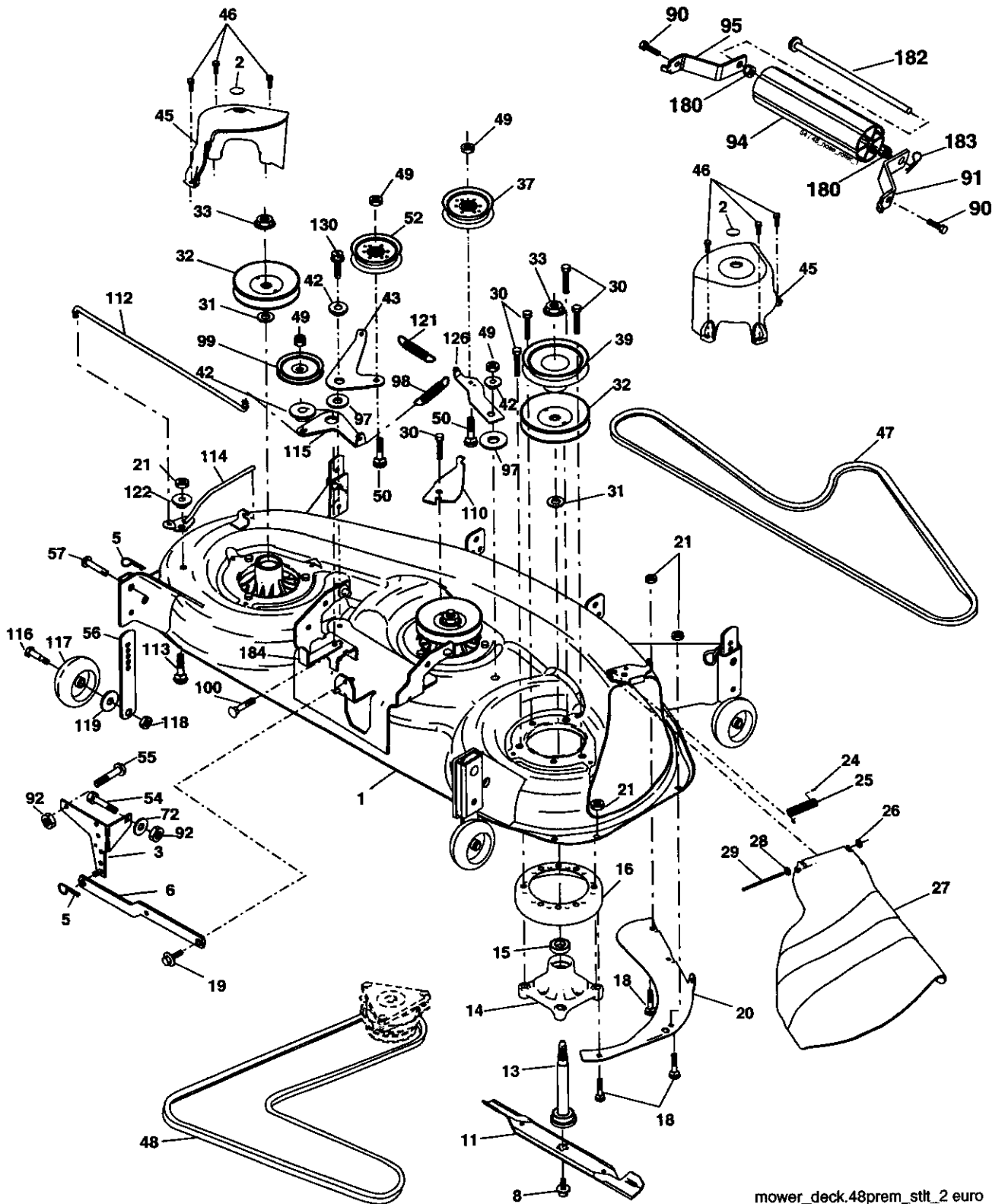
mower_deck.48prem_stlt_2 euro
